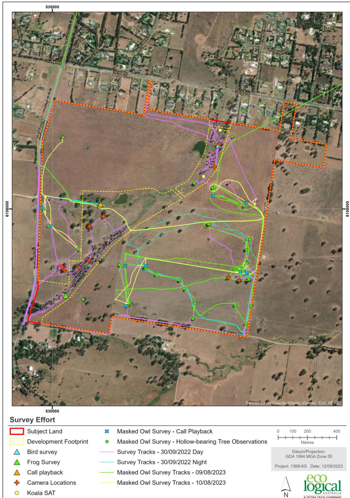
Figure 4 Survey Effort
